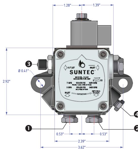
Pump revision 1 - Flange mounting
